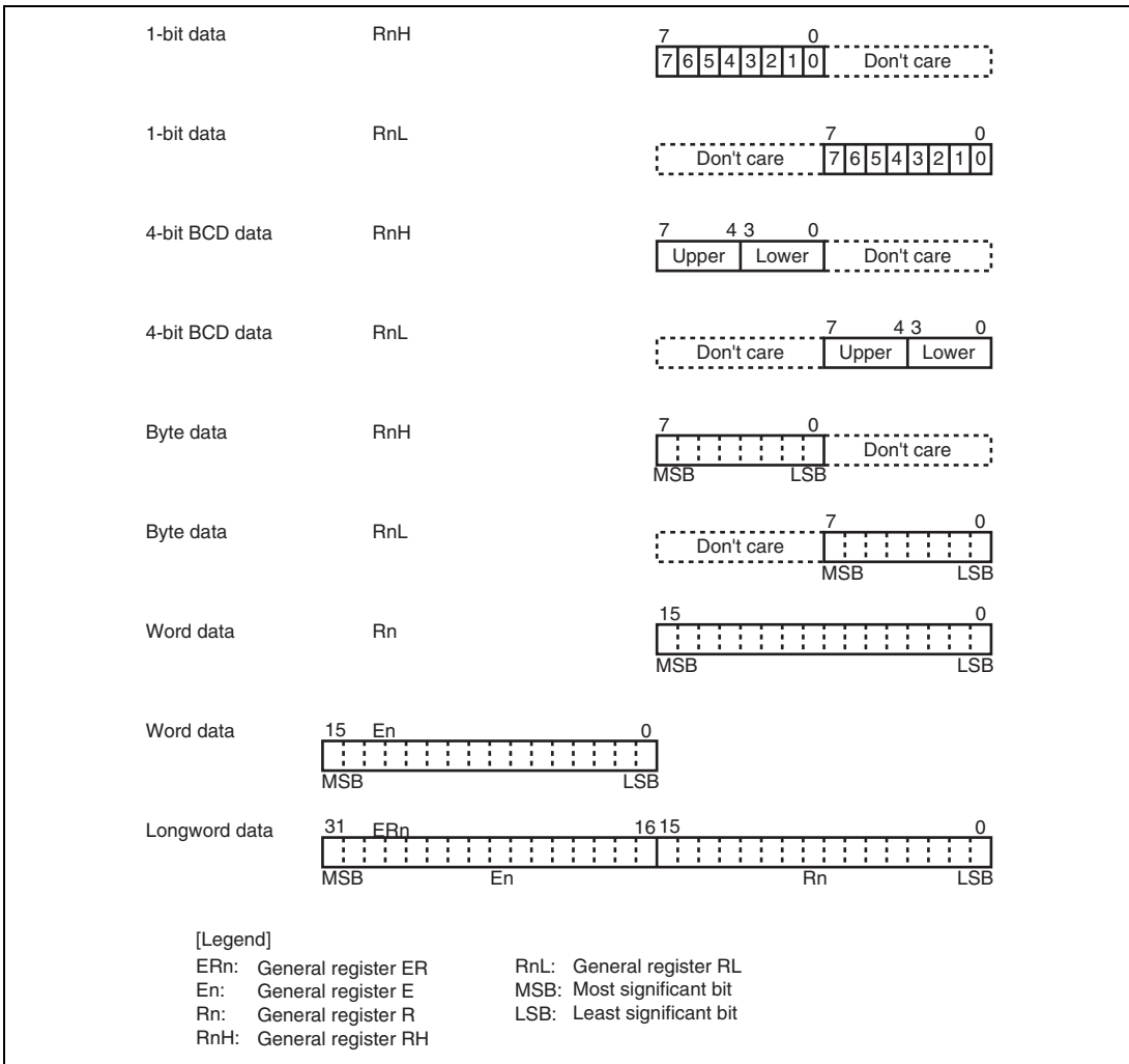
Figure 1.12 General Register Data Formats
