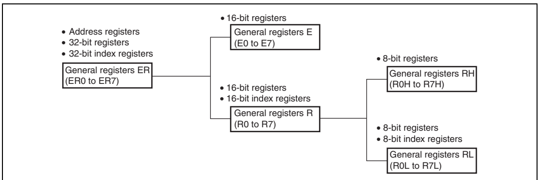
Figure 1.10 Usage of General Registers
