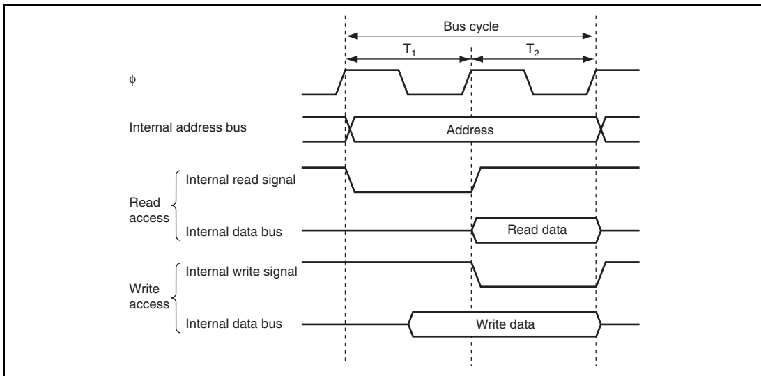
Figure 4.2 On-Chip Peripheral Module Access Timing
