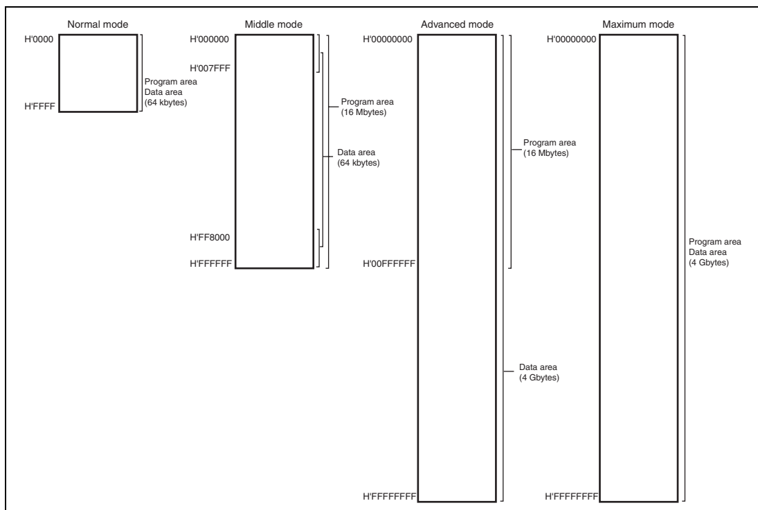
Figure 1.8 Memory Map
