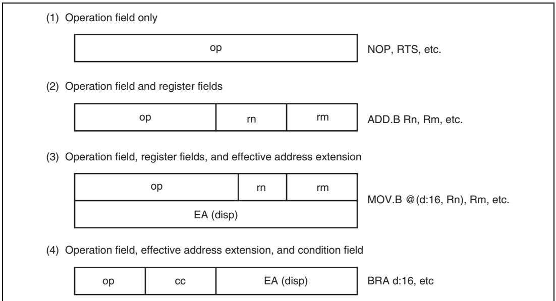
Figure 1.14 Instruction Formats
